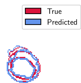
segmentations
